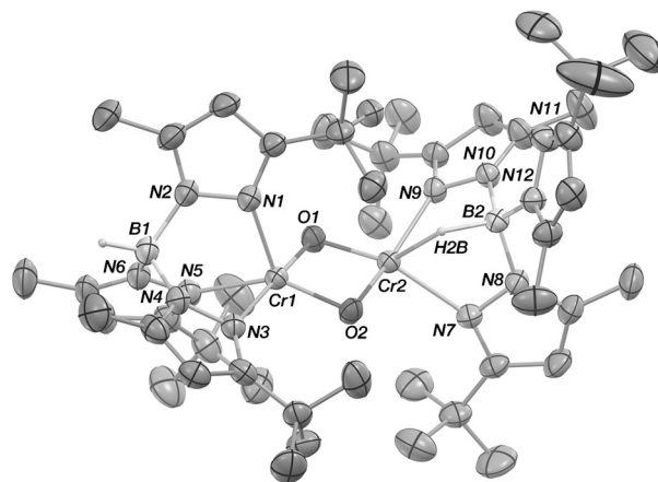
Figure 3. Molecular structure of binuclear 5 (ellipsoids set at 30% probability). Selected interatomic distances [Å] and angles [°]: Cr1–O1 1.9203(15), Cr1–O2 1.7871(15), Cr2–O1 1.7608(15), Cr2–O2 1.8924(15), Cr1–N tp (avg.) 2.158, Cr2–N tp (avg.) 2.154, Cr2–H2B 1.78(2); O1–Cr1–O2 82.38(7), O1–Cr2–O2 83.88(7), Cr1–O1–Cr2 96.07(7), Cr1–O2–Cr2 96.18(7).
